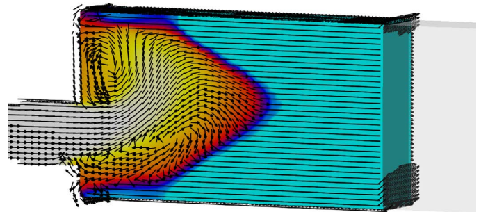
Velocities during start-up for horizontal CC processes
